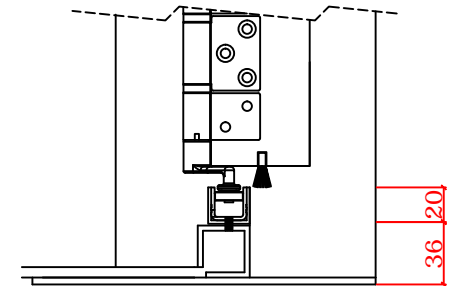
GARAGE/POOL HOUSE SILL
