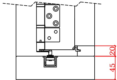
CONSERVATORY SILL w/ WEATHER STOP
